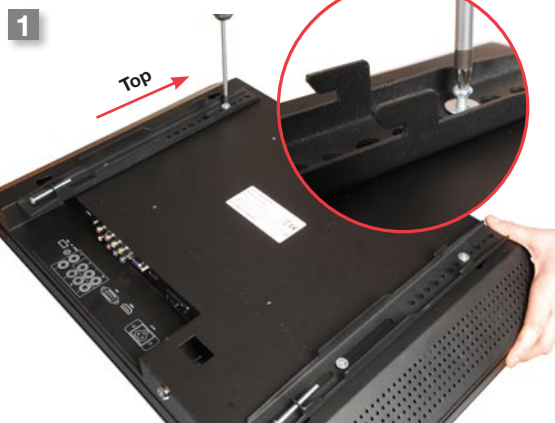
Attach the 2 rails on the LCD screen
